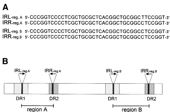
Figure 6. Long DRs, containing IRs, flank regions A and B of plasmid pSB102. (A) The nucleotide sequences of the two 39 bp IRs (IRreg.A and IRreg.B) are given in forward and reverse direction for left and right hand repeats, respectively. (B) Schematic representation of 460 and 301 bp DRs, which contain the left and right hand arms of the 39 bp IRs, respectively. The two pairs of 39 bp IRs are indicated by black arrows. The 460 bp imperfect DR (DR1) is shown as light grey rectangles, the 301 bp DR (DR2) is shown as dark grey rectangles. Region A encompasses nucleotides 3492–7317 of plasmid pSB102 and region B encompasses nucleotides 37587–43160.
