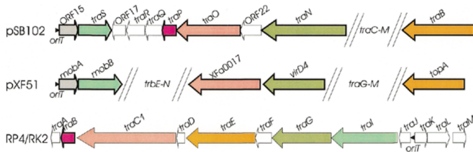
Figure 3. Alignment of the oriT and the Dtr gene region of plasmid pSB102, the X.fastidiosa plasmid pXF51 and IncP-1 \alpha plasmid RK2/ RP4. The Dtr genes are shown as arrows. Genes encoding similar products are displayed in the same color. ORFs of unknown function or genes without a similar product in the pSB102 Dtr gene region are shown as white arrows. Genes displaying highest identities of their deduced amino acid sequences are indicated by bold lines. GenBank accession numbers of the respective nucleotide sequences are as follows: X.fastidiosa plasmid pXF51, AE003851; IncP-1 \alpha plasmid RK2/ RP4, L27758.
