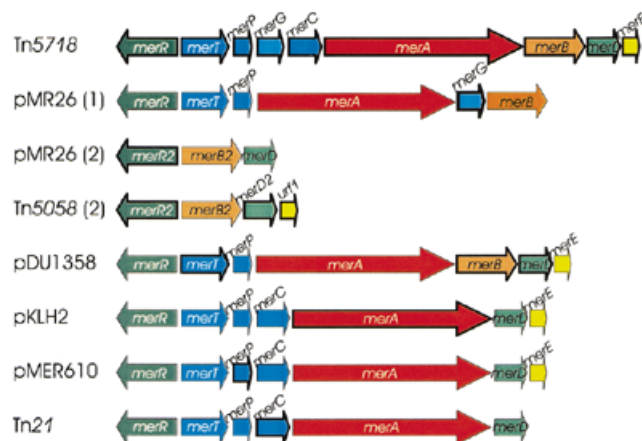
Figure 5. Alignment of various mer operons mediating resistance to inorganic mercury and organomercurials located on plasmids and transposons. Genes displaying highest identities of their deduced amino acid sequences are indicated by bold arrows. Regulatory genes are shown in green, transfer genes in blue, enzyme genes in red and genes of unknown function in yellow. GenBank accession numbers of the respective nucleotide sequences are as follows: Pseudomonas sp. K62 pMR26 mer operon 1, D83080; pMR26 mer operon 2, AB013925; Pseudomonas sp. ED23-33 mer operon 2, Y17897; Serratia marcescens plasmid pDU1358, M24940 and M15049; A.calcoaceticus plasmid pKLH2, AF213017; Ralstonia sp. plasmid pMER610, Y08993; Tn21, AF071413.
