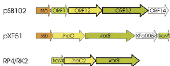
Figure 4. Alignment of genes in the maintenance (Mai) region of plasmids pSB102, pXF51 and RK2/RP4. Putative Mai genes are shown as arrows. Genes encoding similar products are displayed in the same color. ORFs of unknown function are shown as white arrows. Genes displaying highest identities of their deduced amino acid sequences are indicated by bold lines. GenBank accession numbers of the respective nucleotide sequences are as follows: X.fastidiosa plasmid pXF51, AE003851; IncP-1 \alpha plasmid RK2/RP4, L27758.
