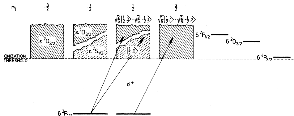
FIG. 1. Autoionization states and continuum states reached from the ground state 6^2P_{1/2} of thallium with circularly polarized \sigma^+ light.
