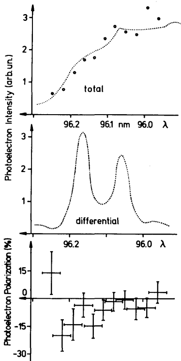
Fig. 6. Photoionization of N_2O at the threshold: (top) measured photoelectron intensity ( \circ , 17 ....., 20 ); (center) differential photoelectron spectrum measured by Ref. 21; (bottom) measured spin polarization of photoelectrons. 17
