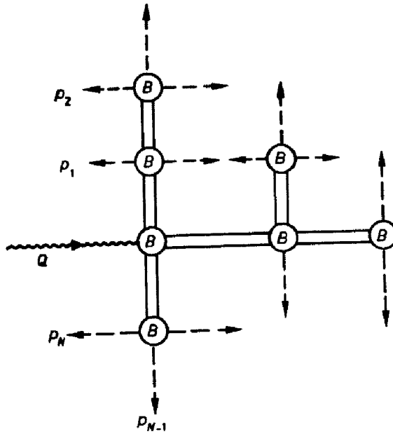
Fig. 3. - Full bootstrap decay.
