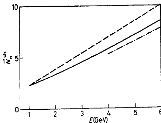
Fig. 4. - Charged-pion multiplicity as a function of e^+e^- energy, for allowed final states consisting of pions only (---), pions and kaons (—) and pions, kaons and nucleons (-.-.-).
