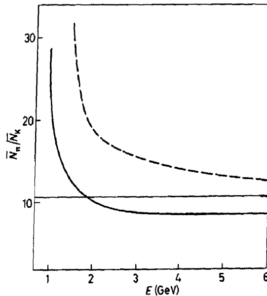
Fig. 8. - Ratio of pion to kaon multiplicities as a function of e^+e^- energy with (—) and without (---) G -parity conservation.
