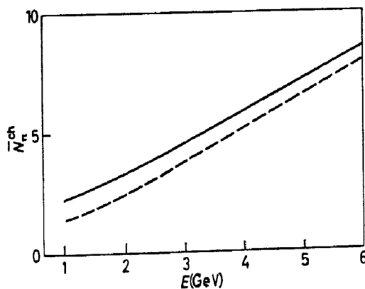
Fig. 10. - Charged-pion multiplicity, allowing pions and kaons in the final state, for full bootstrap (---) and linear cascade (—).
