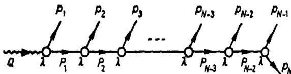
Fig. 2. - Linear cascade decay.
