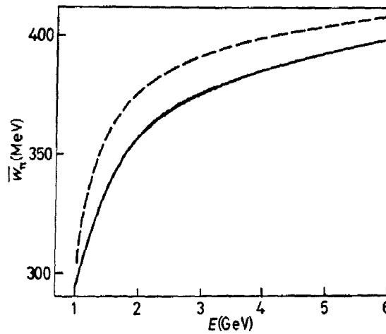
Fig. 7. - Average pion energy as a function of e^+e^- energy for full bootstrap (---) and linear cascade (—).
