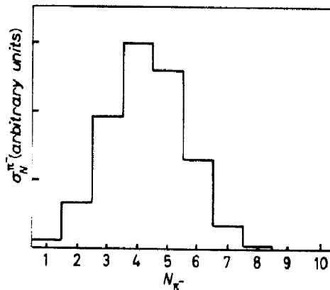
Fig. 9. - Multiplicity distribution for negative pions, allowing pions and kaons in the final state, at an e^+e^- energy of 6 GeV.
