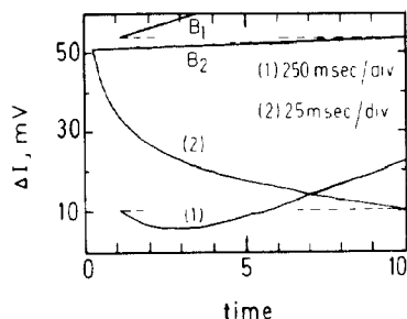
FIG. 1. Chemical relaxation spectrum (section t \geq 5 msec) of AcCh receptor from T. californica , at 1 mM Ca, 23.5°, after a temperature jump of 3.5°. \Delta I measures light intensity changes at 480 nm. 10 mV correspond to an absorbance change of 0.0005 per 0.7 cm. Double-sweep oscilloscope record at two time scales; B 1 and B 2 are reference tracings (no temperature jump). The pre-amplitude of 578 mV ( t \leq 5 msec) was electronically suppressed, and cooling correction was applied.
