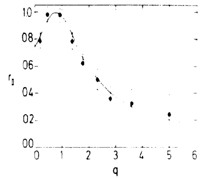
FIG. 3. The ratio r_{11} = (\tau_{11} - \tau_2) / (\tau_{11}^m - \tau_2) as a function of q , plotted according to Eq. 11. See text.
