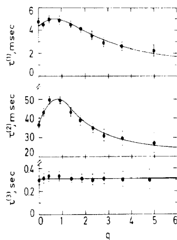
FIG. 2. Kinetic titration with AcCh of AcCh receptor from T. californica . Plot of time constants \tau^i of the Ca-AcCh receptor relaxation at 1 mM Ca and 23.5° as a function of q = [A^0]/[R^0] , where [A^0] is the (variable) total concentration of AcCh and [R^0] is the (practically constant) total concentration of AcCh binding sites of AcCh receptor ( 5 \times 10^{-6} M). See text.
