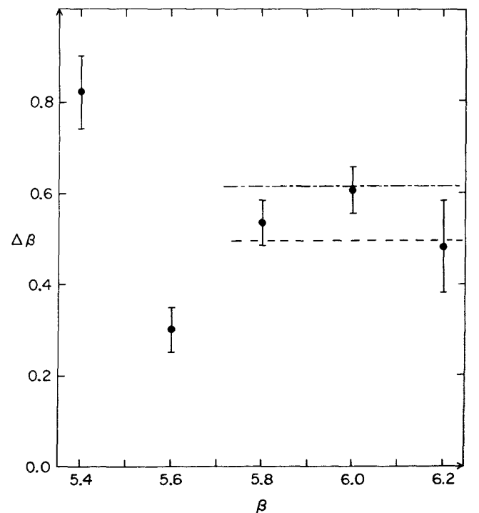
FIG. 1. \Delta\beta as a function of \beta for QCD with three light dynamical flavors. The dashed line shows the asymptotic-scaling prediction of Eq. (5). Also shown above it is the asymptotic-scaling prediction for the quenched theory.
