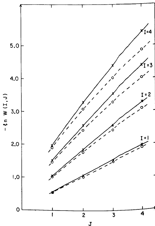
FIG. 2. -\ln W(I, J) as a function of J for various I . The crosses show the pure SU(3) of Ref. 2 at \beta = 5.8 while the circles display our data at \beta = 5.6 for the theory with three light dynamical flavors. The error bars on all the points are smaller than or comparable to the size of the points themselves.
