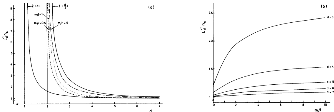
FIG. 1. The ratio of the critical density in terms of L_d^{-1} n_c of a Bose gas to the corresponding Boltzmann gas (a) in relation to the spatial dimensions d for various stated values of the parameter m\beta , and (b) as a function of m\beta for the listed d .
