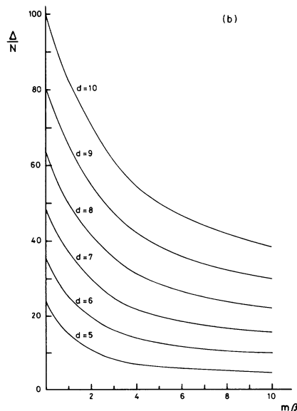
FIG. 2. The jump in specific heat per particle \Delta/N at T_c (a) in relation to the spatial dimensions d for given values of m\beta , and (b) as a function of m\beta for the stated d .
