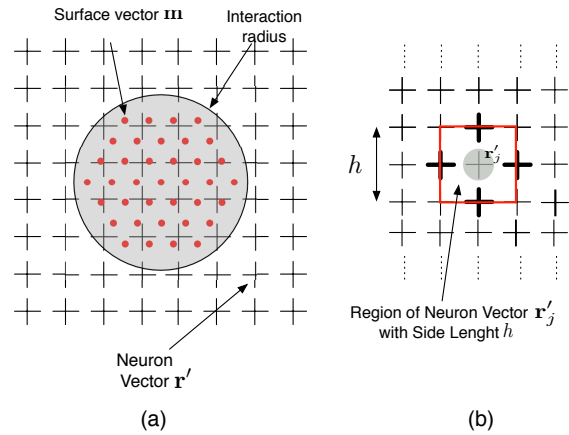
Figure 8: (a) Result of transforming neuron locations into a 2-d vector space. The transformation enables to extract neighboring relations between surface vectors (red dots) and transformed SOM neurons (black cruces) in order to determine hyperspheres radii in exploration space. (b) Region of a neuron vector \mathbf{r}'_j (red quad).
