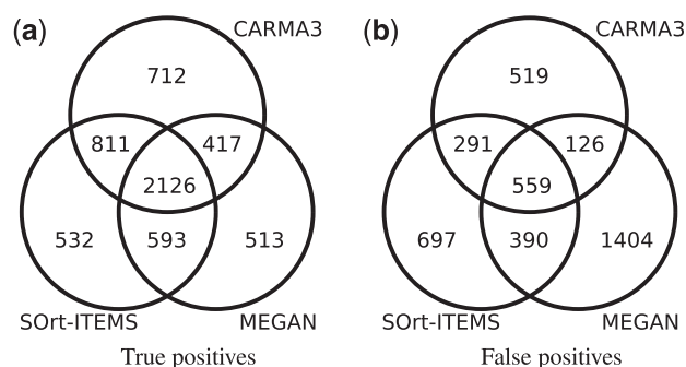
Figure 2. Overlap of 25 000 simulated metagenomic reads classified by CARMA3, SOrt-ITEMS and MEGAN for the order-filtered data set at taxonomic rank class.
