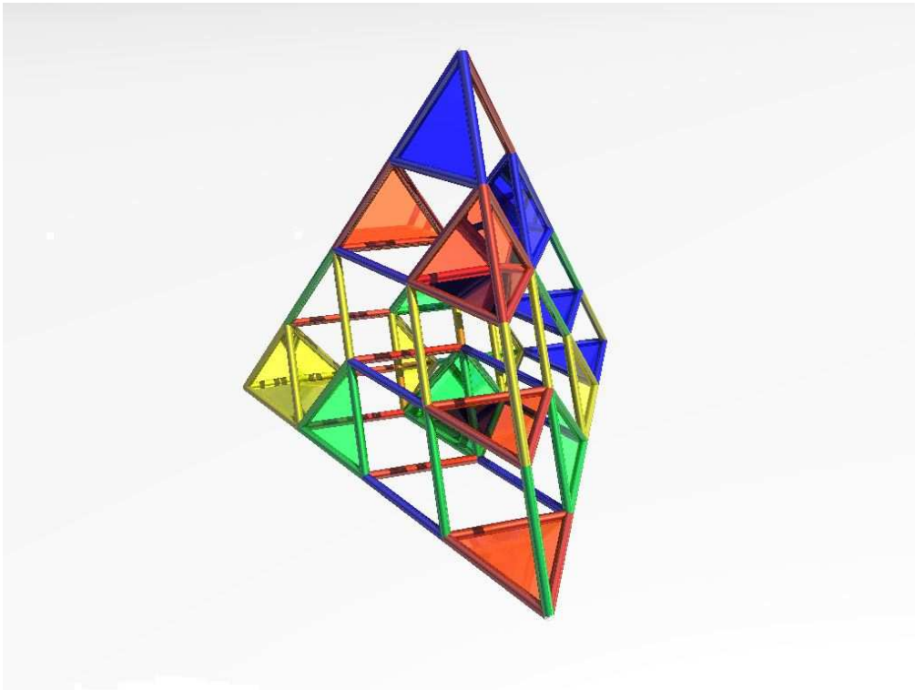
Figure 6.1: The canonical representation of FourFour
