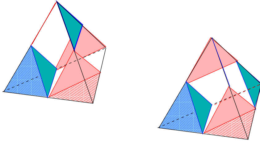
Figure 2.1: The sum of two prisms for n = 4
