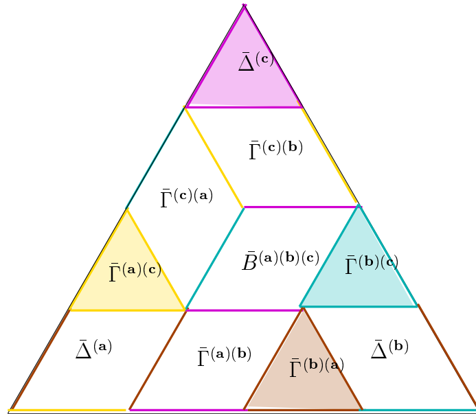
Figure 2.4: The Dual Marriage
