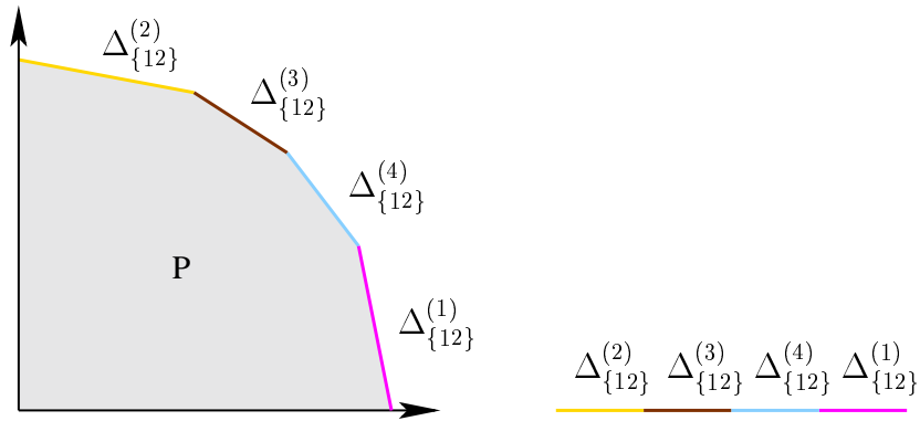
Figure 2.2: The dual surface and its canonical representation
