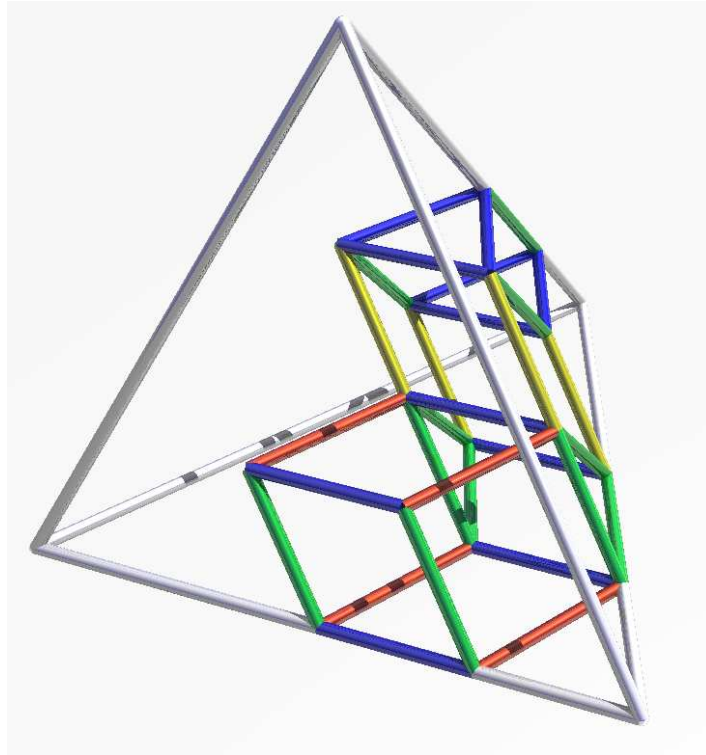
Figure 6.2: The Tentacle of Example 6.8
