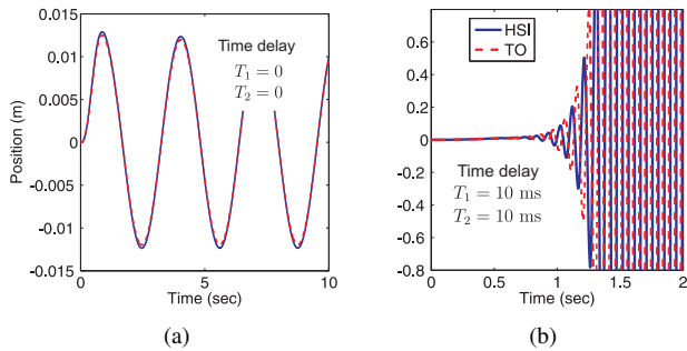
Fig. 3. Simulated HSI and TO position for the standard control architecture from Fig. 2 without time delay (a) and with time delay T_1 = T_2 = 10 ms (b): Even a small time delay can lead to instability.
