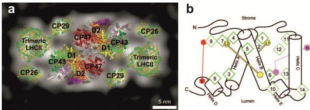
Figure 2: PS II-LHCII supercomplex and the monomeric LHCII protein-model (Harris, 2009; Nield and Barber, 2006). a. Top view of the PSII-LHCII supercomplex. Overlaid X-ray structures of the PS II core (Ferreira et al., 2004) without extrinsic OEC proteins, and the spinach LHCII complex (Liu et al., 2004), onto the luminal top view of the 3D structure of the spinach PS II –LHCII supercomplex derived from cryo-EM and single particle analysis (Nield et al., 2002). The transmembrane helices of the D1 (yellow), D2 (orange), CP43 (green), CP47 (red), and \alpha - and \beta -subunits of cytochrome b 559 (purple) subunits are displayed as ribbons b. Schematic of the LHCII protein. Transmembrane (A–C) and amphipathic (D–E) helices are shown as cylinders (Liu et al., 2004). Chlorophyll chl a (Chl 1–8) and chl b (Chl 9–14), represented by diamonds and dotted diamonds, respectively. Two luteins (L1 and L2, yellow), one 9'- cis -neoxanthin (N, pink), and one violaxanthin (V, red) are displayed.
