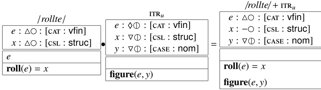
Figure 15: Combining monosemous rollte with underspecified \text{ITR}_u .
