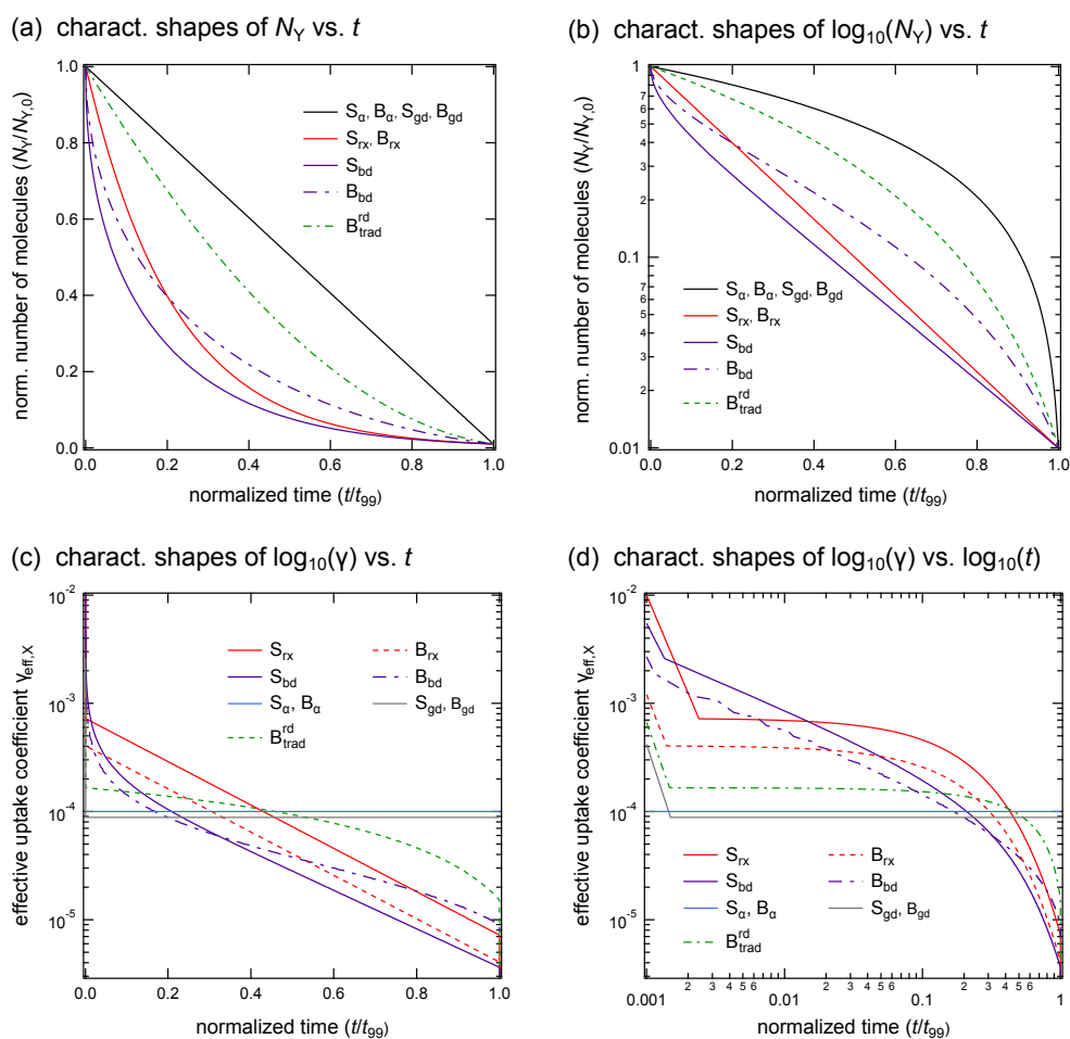
Fig. 5. Normalised representation of the decay shapes of the total amount of Y ( N_Y , panels a and b ) and the effective reactive uptake coefficient ( \gamma_{\text{eff},\text{X}} , panels c and d ) for all limiting cases on linear and logarithmic time scales (see Sect. 5.1 for a more complete description). In addition to the eight regular limiting cases, we also display the traditional reacto-diffusive case, B_{\text{trad}}^{\text{rd}} . Note that B_{\text{trad}}^{\text{rd}} is not a limiting case, but a distinct scenario in the reaction-diffusion regime.
