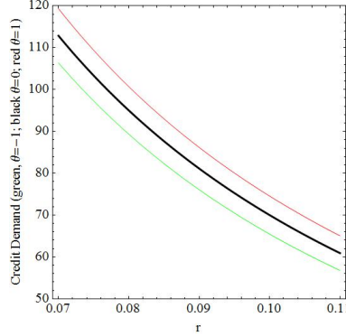
Figure 4: credit demand n^s = 1 (black \rightarrow \varepsilon = 0 , red \rightarrow \varepsilon > 0 , green \rightarrow \varepsilon < 0 )
