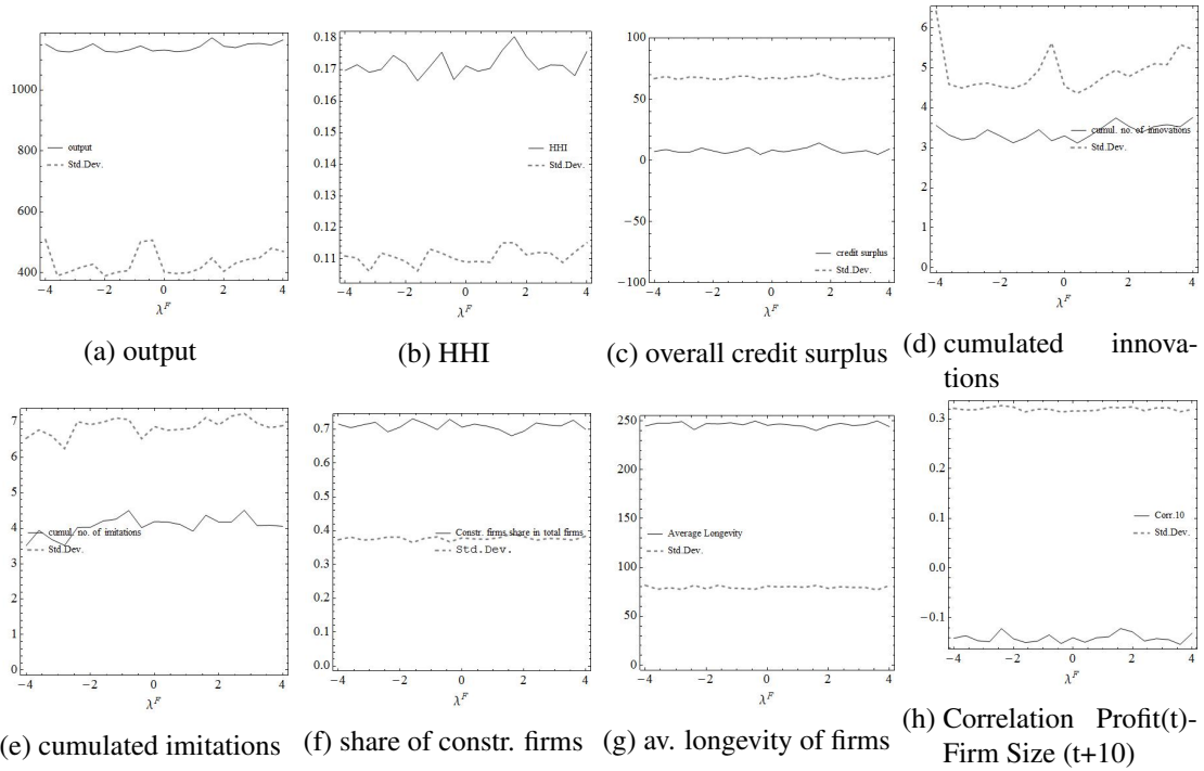
Figure 8: Impact of firm rule
