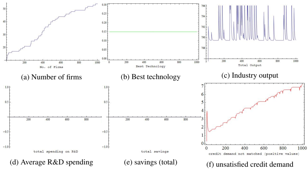
Figure 2: Representative over time evolution with no credit available.
