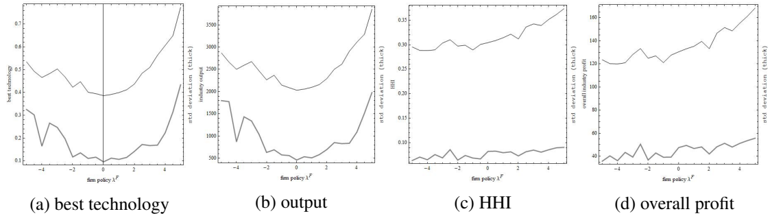
Figure 9: Effect of firm rule with abundant credit supply
