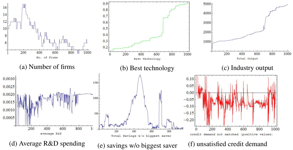
Figure 3: Representative over time evolution with credit available l^s = 0.3 .
