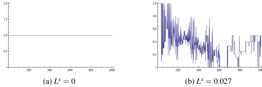
Figure 5: Share of firms that face constraints in financing over time
