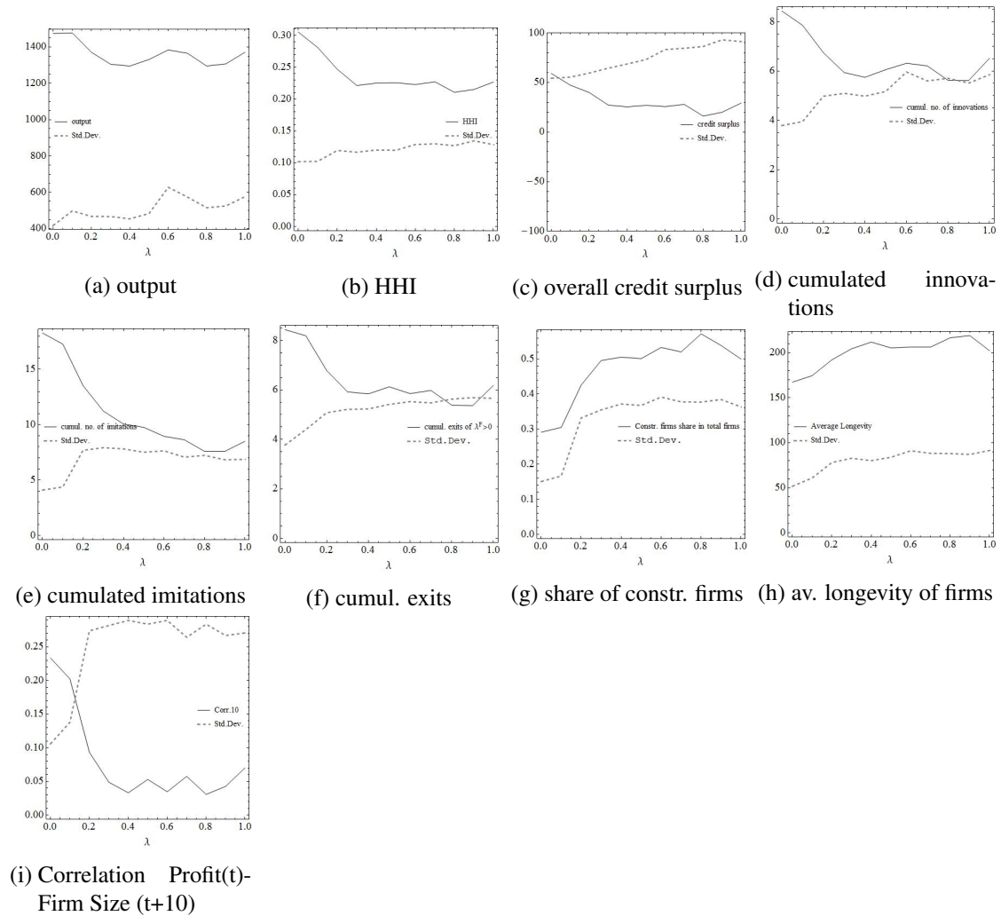
Figure 7: Impact of bank policy
