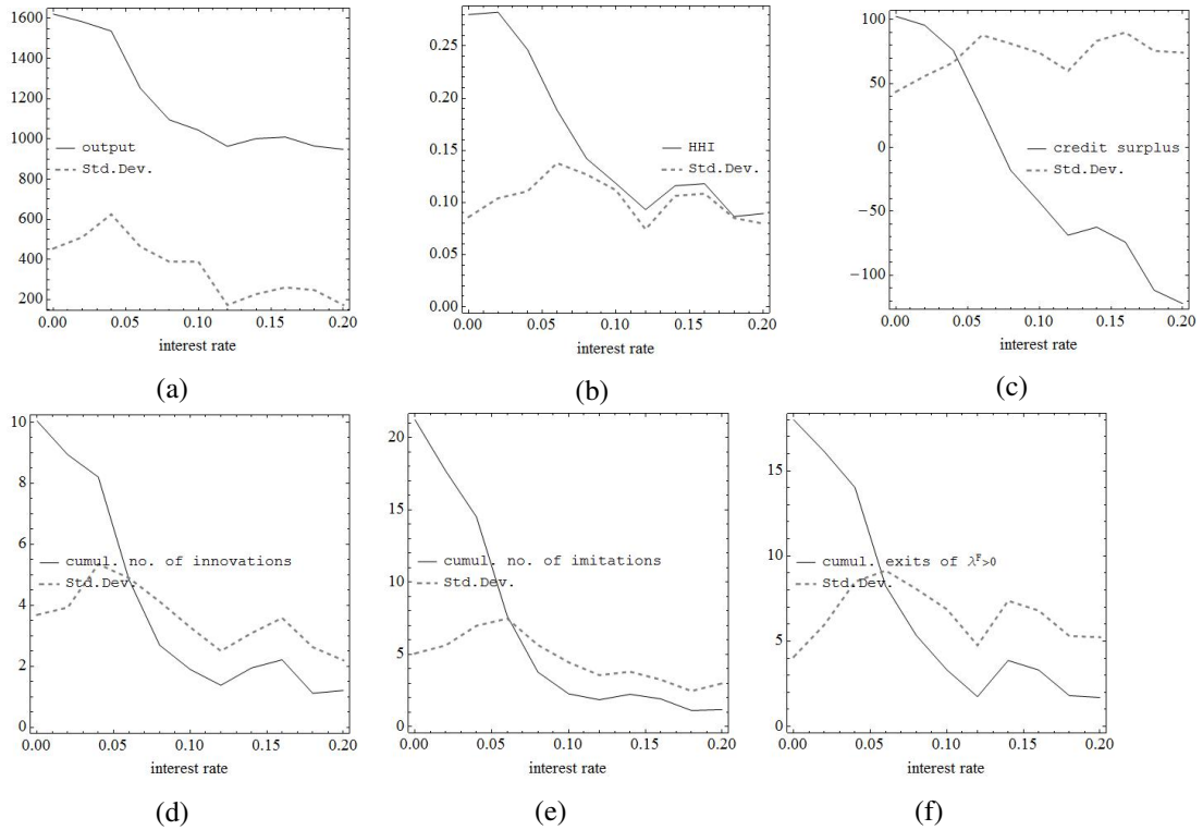
Figure 6: Impact of the interest rate
