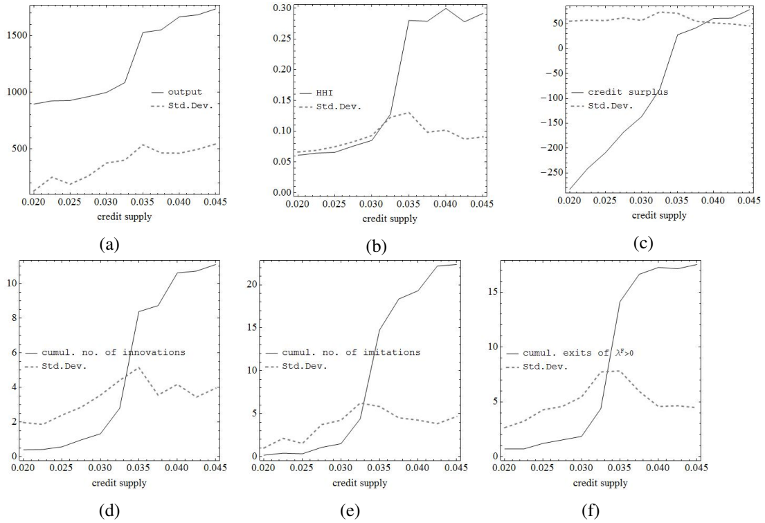
Figure 4: Impact of credit supply
