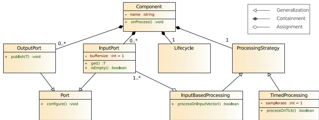
Figure 7.1.: Class diagram of the programming model, focused in the component level.
