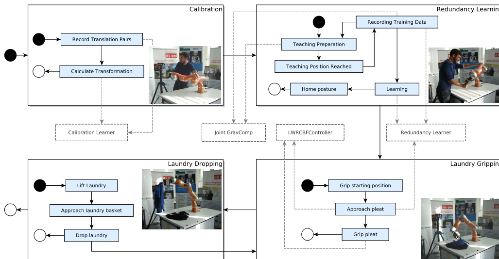
(b) States are shown in blue , black arrows represent Transitions, gray-dashed arrows indicate links to the structural model ( black-dashed ), either as Condition for Transitions, or triggering different learning states in the Adaptive Modules.
