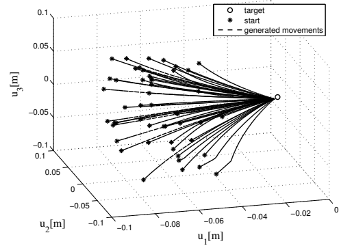
(b) Left hand trajectories generated with a motion primitive from various starting points to the same target point.
