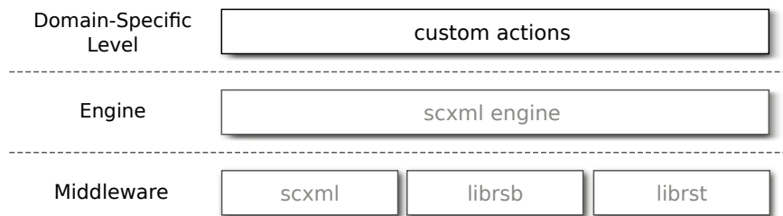
Figure 7.5.: Technology mapping for the behavioral aspects with the custom actions for motion primitive architectures realized based on an SCXML engine that extends the Apache SCXML engine with connections to the librsb middleware and the librst type library. Libraries in light gray boxes were not implemented as part of this work.
