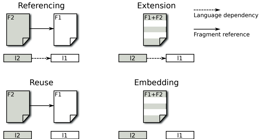
Figure 2.2.: Language and fragment dependencies in the different types of language modularization [Völter et al., 2013, Section 4.6].
