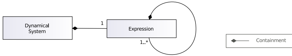
Figure 5.12.: Metamodel, focused on the algorithmic aspects.
