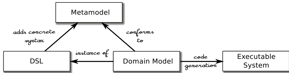
Figure 1.2.: A typical modeling approach with DSLs: The DSLs add a concrete syntax to a metamodel and are used to implement a concrete domain model. Code generation is one approach to make the domain models executable.
