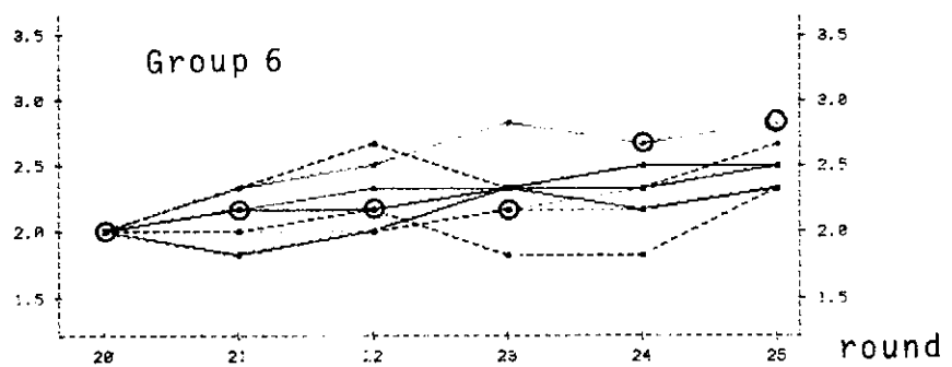
Figure 3: Group means of intended deviation times in the experiment (o) and in 8 Monte-Carlo-simulations.
