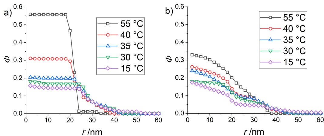
Figure 5. (a) Density profiles of the H-pNIPMAM-core with a CCC of 10 mol% in D 2 O (data adapted from Cors et al. 35 (b) Density profiles of the core monomers of the H-pNIPMAM-core D7-pNIPMAM-shell system with the same core as in (a) and an index-matched shell (CCC = 1.9 mol%).
