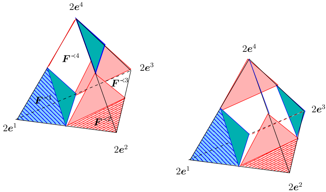
Figure 4.2: The sum of two deGua Simplices for n = 4
