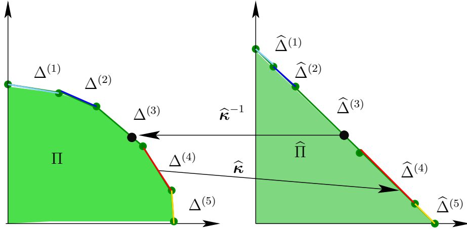
Figure 4.1: Mapping \partial\Pi onto \widehat{\Delta}
