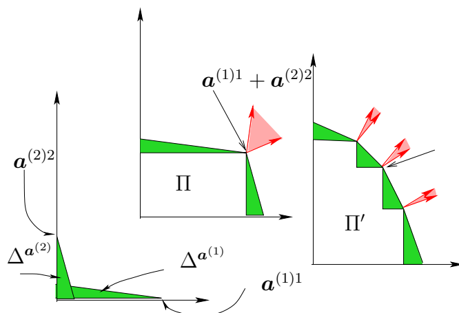
Figure 1.2: Construction of global plans
