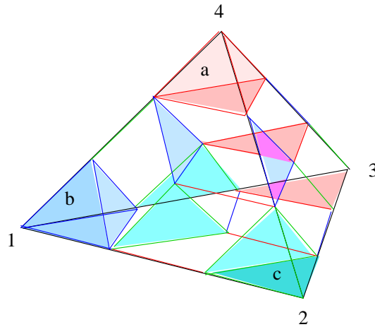
Figure 6.3: A circle of 3 deGua Simplices in 4 dimensions.
