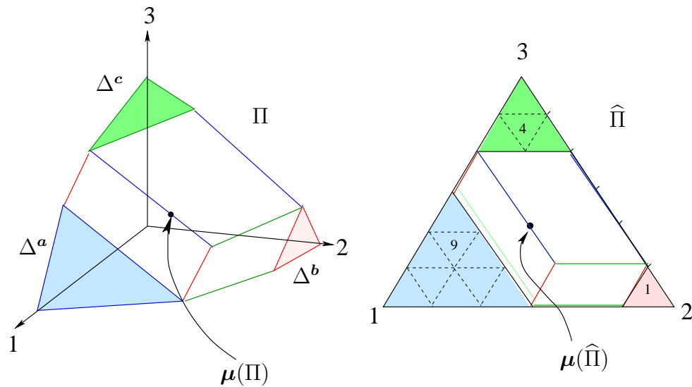
Figure 5.3: The \mu\pi solution for (l_a, l_b, l_c) = (3, 1, 2)
