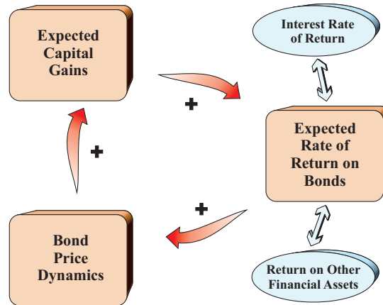
Figure 5: Blanchard-type bond-market instability [Boundedness by interacting "naive" and "rational" endogenous opinion formation]
