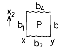
Fig. 7. Illustration to equation (5.3)
