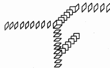
Fig. 5. Part of a \Gamma -vortex (for example \Gamma = Z_3 ), which splits
