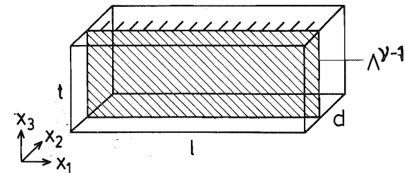
Fig. 6. Vortex container \Lambda^3 with sublattice \Lambda^2 . The container is as in Fig. 4
