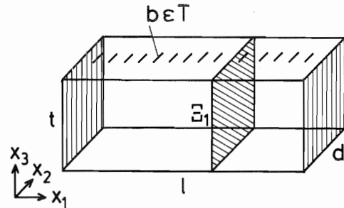
Fig. 4. Vortex container in 3 dimensions, equivalent to that of fig. 3. The righthand face and the lefthand face (hatched) are to be identified. E_1 is a cross-section of the container. If one identified the other faces pairwise, one gets a torus T^3
