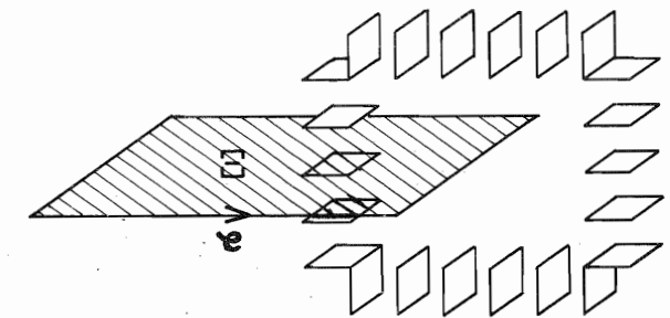
Fig. 2. Vortex in 3-dimensional Z_2 lattice gauge theory, winding around a path \mathcal{C} = \partial \Xi .
