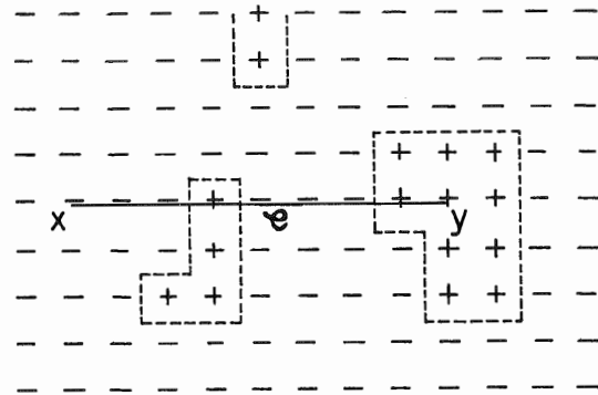
Fig. 1. Peierls contours (dotted lines) in 2-dimensional Ising model. Lattice points x and y are linked by a path \mathcal{C}
