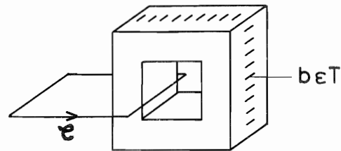
Fig. 3. Vortex container A in 3 dimensions, which winds around the path \mathcal{C} . On the boundary of A the set T is marked
