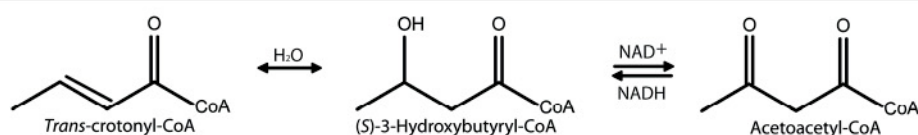
Figure 1 Enoyl-CoA hydratase and ( S )-3-hydroxyacyl-CoA dehydrogenase reactions of FA degradation pathway, catalyzed by FadB'.
