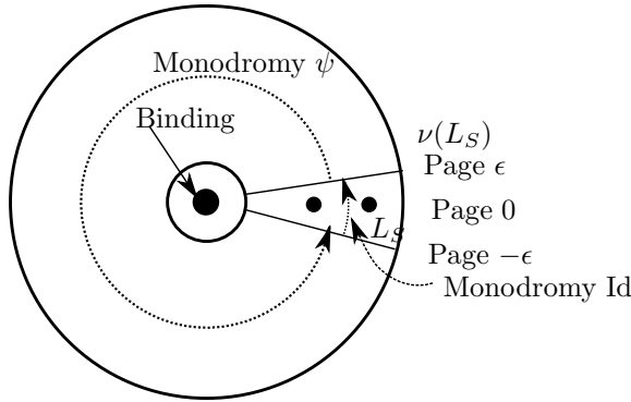
FIGURE 8. Pages around a Legendrian sphere.
