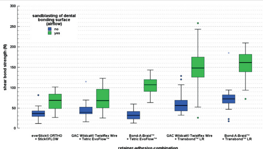
Figure 3 Shear bond strengths (SBS) of the retainer-adhesive-combinations tested with and without prior sandblasting. Boxplots show median and interquartile range while whiskers denote the data range. ° outliers (>1.5 x IQR beyond upper/lower quartile); * extreme values (>3 x IQR beyond upper/lower quartile).
