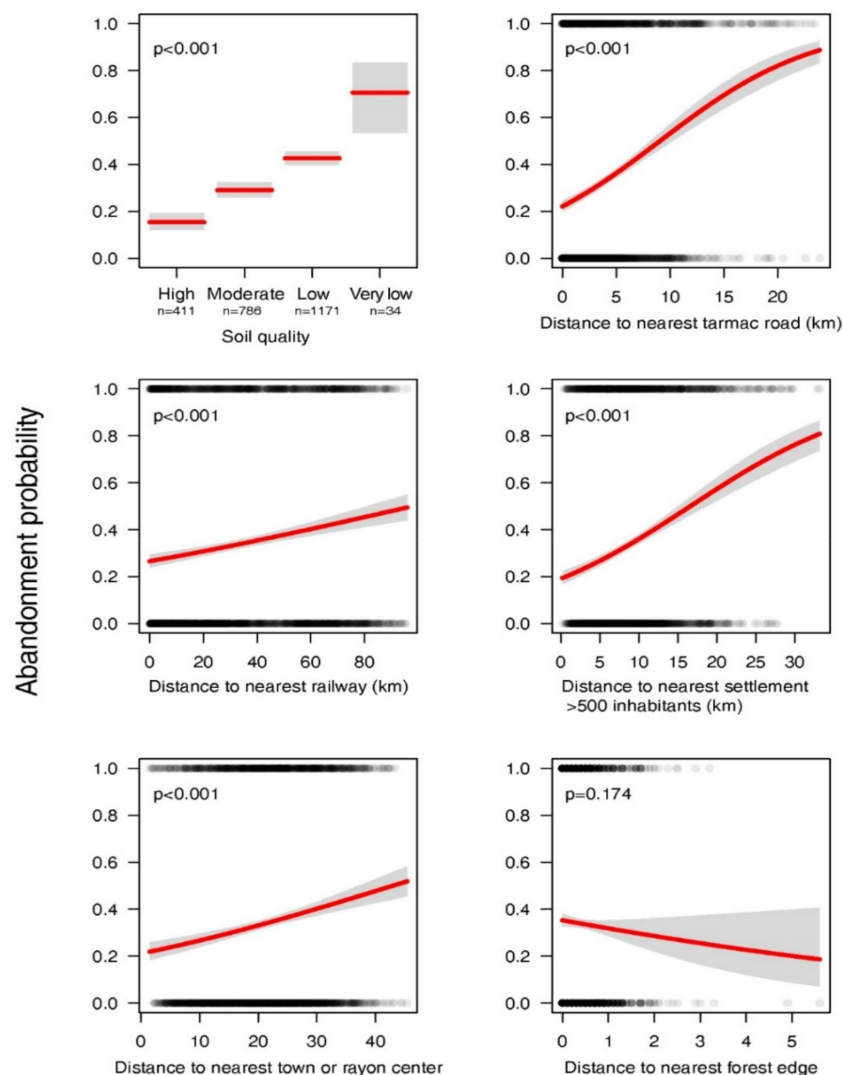
Figure 2. Predictions of cropland abandonment probability from univariate logistic regression models. p -values indicate significant associations between abandonment probability and the respective variable. Models are plotted with standard errors (grey intervals). The data is overplotted (0—samples of stable cropland, 1—samples of abandoned cropland).
