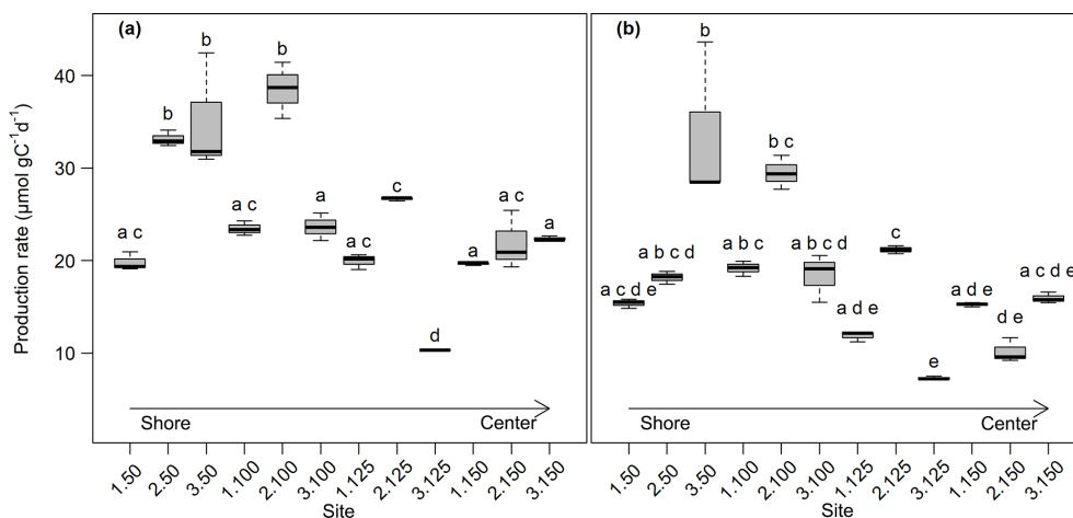
Figure 3. CO 2 (a) and CH 4 (b) production rates at 0–5 cm sediment depth ( n = 3 ). Production rates were calculated from the linear regression of concentration increase over time. Bold lines are the median, boxes show the 25 and 75 percentile, and whiskers indicate minima and maxima within 1.5 times the interquartile range. Identical lowercase letters indicate production rates that were not significantly different (i.e., p > 0.05 ) from each other.
