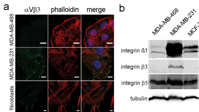
Fig 6. Expression of \beta -integrin subunits in human breast cancer cell lines. The expression of, \alpha V \beta 3-, \beta 1-, \beta 3-, and \beta 5- integrin in MDA-MB-468, MDA-MB-231 and MCF-7 cells was studied by confocal immunofluorescence ( \alpha V \beta 3) (a) or western blotting ( \beta 1-, \beta 3-, \beta 5-) (b), respectively, as described in Figs 3 and 5. Only MDA-MB-231 cells showed expression of ( \alpha V) \beta 3-integrin, in partial colocalization with actin stress fibers in a fibroblast-like pattern. All breast cancer cell lines studied expressed \beta 1-, and \beta 5- integrin subunits (b), albeit in different quantities.
