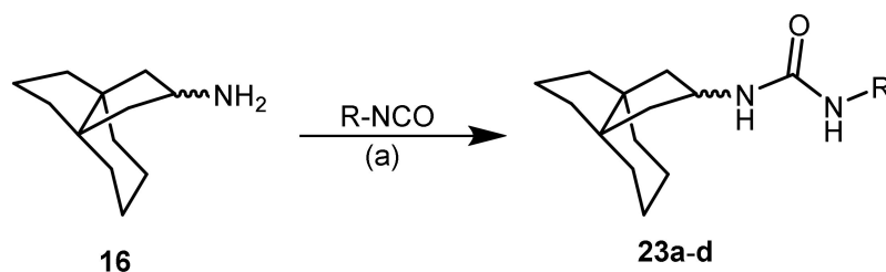
Scheme 4. Synthesis of propellane-based urea derivatives 23 . Reagents and reaction conditions: (a) \text{R-N=C=O} , \text{Bu}_2\text{Sn(OAc)}_2 , THF, rt, 24–48 h, 22–91%. Since a 1:1-mixture of diastereomeric primary amines 16 was used as starting material, 1:1-mixtures of urea 23 were obtained. The residues R are defined in Table 3.
