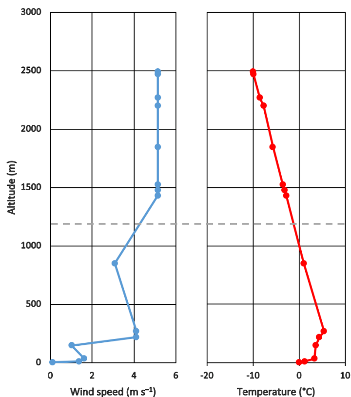
Figure 2. Composed wind speed and temperature profile for Münster, 5 December 2018, 00:00 UTC; dashed line: maximum height of the model domain (1200 m).
