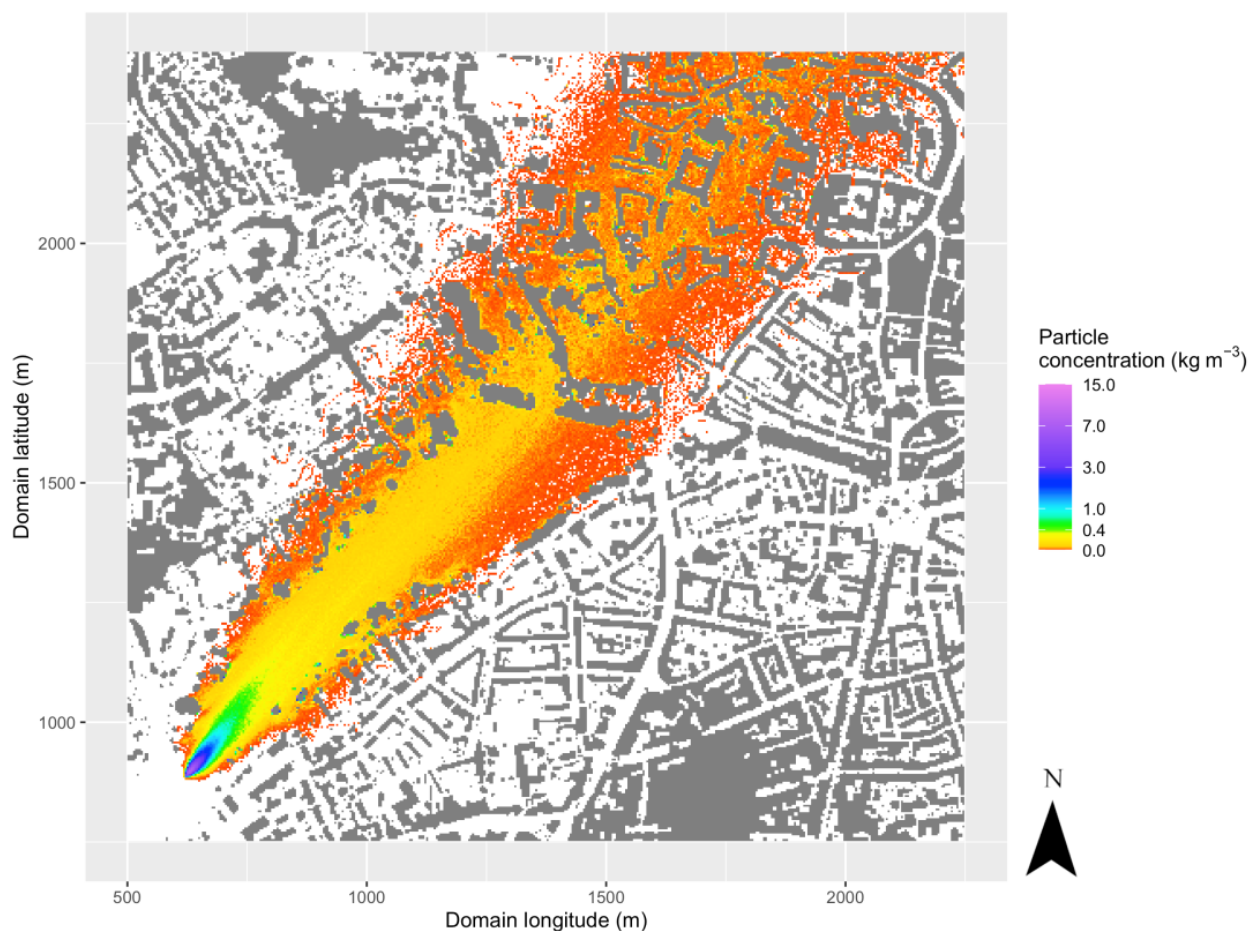
Figure 7. Particle dispersion in the area of interest above the city center at an altitude of 18 m (grey: topography; white: street canyons and open spaces without particles).
