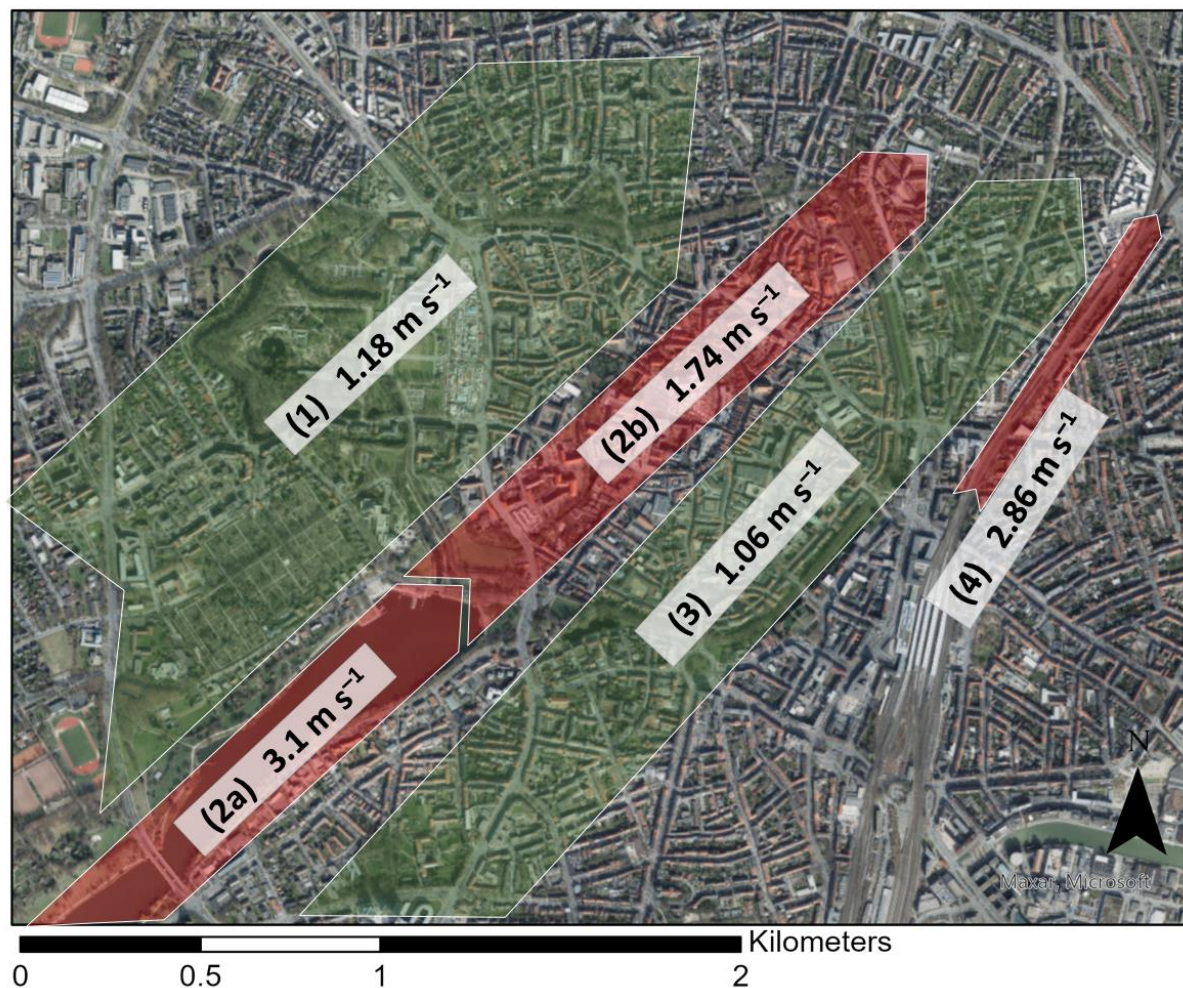
Figure 4. Wind aisles and their mean wind speed at an altitude of 26 m above domain minimum (ADM).
